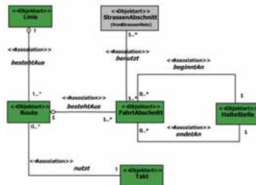
Fig. 10: Extract of the VVU data model (UML-notation)
