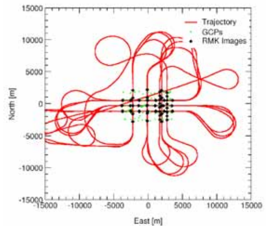
IGI AEROcontrol II d test flight Vaihingen/Enz (June 9, 2000).
