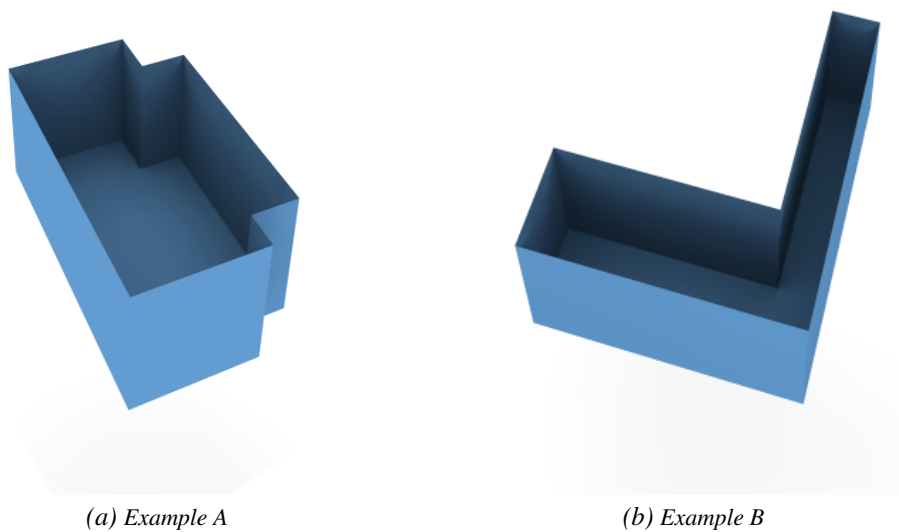
Figure 5.11: Models obtained through the application of the automatic reconstruction technique using as inputs the sub-clouds described in Example A (a) and B (b).
