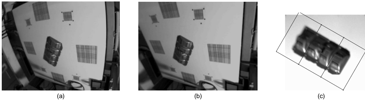
Figure 3: (a) Original image taken with the overview camera. (b) The same image after correction of lens distortion. (c) Again, the same image after rectification. Each image pixel now corresponds directly to a certain metric area on the ground plate. The object is segmented and three locations for the stereo camera are generated.
