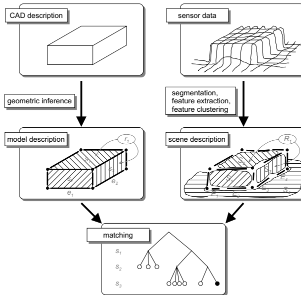
Figure 7: Typical object recognition system. The left part of the diagram can be solved in advance (off-line) whereas the right part has to be solved each time a new object is to be recognized (on-line).
