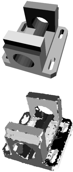
Figure 10: Segmented surface description obtained from the CAD model (above) and result of segmentation of the merged sensor data into planar faces (below).
