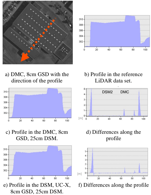
Figure 3: Profiles of the industrial building and their errors along the profiles..
