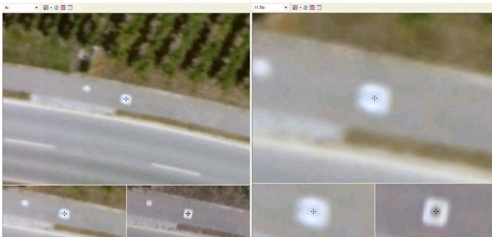
Fig. 6: Influence of the de-focused DigiCAM camera head no. 125 on GCP no. 3041029, 4x zoom (left), 11,7x zoom (right). Each with the left and right image for stereo display (below).
