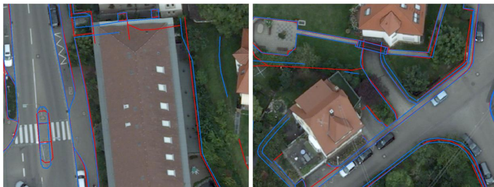
Fig. 11: Line measurements in 8cm GSD images for RMK (red) and DMC (blue). Background image: UCX orthophoto, 8cm GSD.
