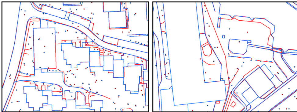
Fig. 7: Left: Area 2 "High Riser", comparison of stereoplottling results 8cm GSD (red) to 20cm GSD (blue), RMK. Right: Area 1 „Inner City“, comparison of stereoplottling results 8cm GSD, UCX (red) to DMC (blue).
