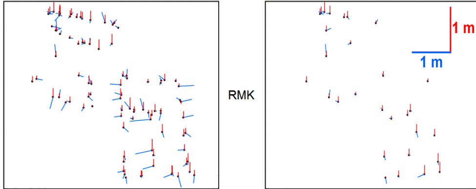
Fig. 8: Differences of all point measurements (left) and manhole cover measurements (right) for RMK, 8cm GSD compared to 20cm GSD for Area 2 and 3. Differences dx and dy (blue), dz (red).
