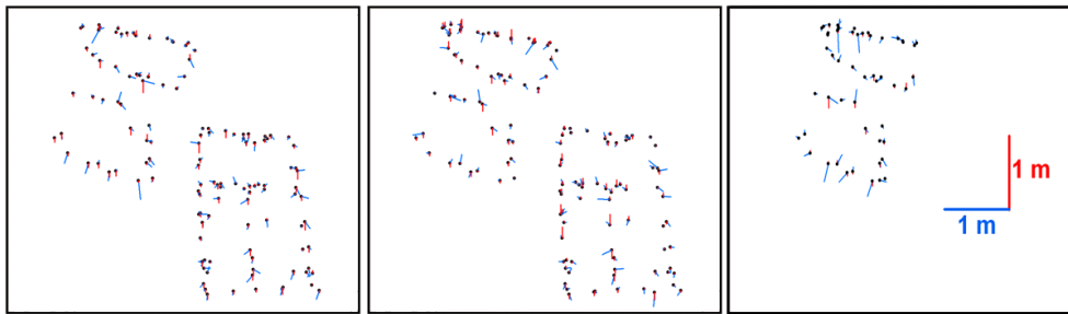
Fig. 9: Differences of all point measurements for Area 2 and 3 in 8cm GSD . From left to right: RMK-DMC, RMK-UCX and RMK-DigiCAM (only northern Area 2). Differences dx and dy (blue), dz (red).
